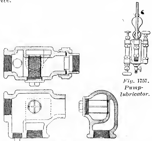
Figs. 1758-1760. Sections.
